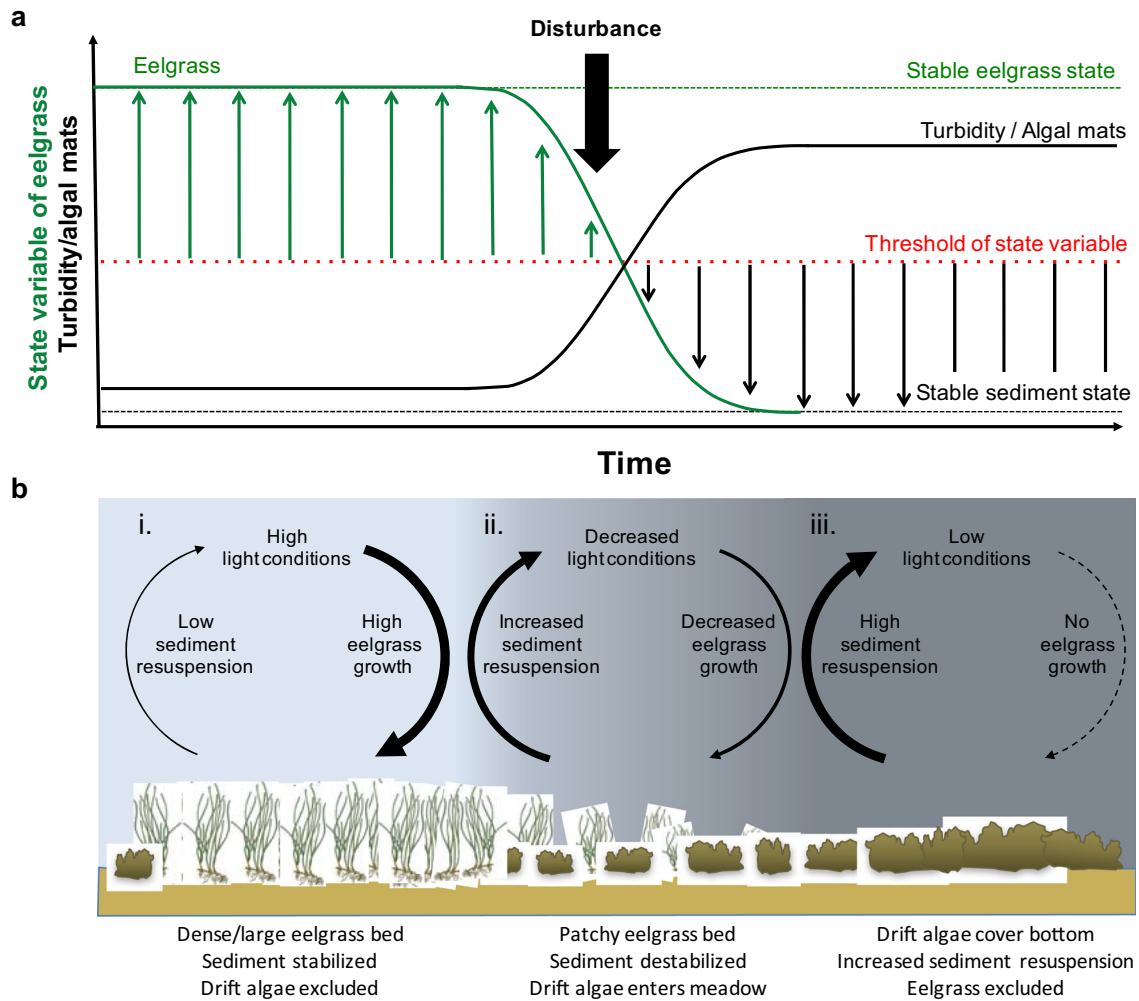
Fig. 8 Conceptual model (a) and schematic illustration (b) of self-amplifying feedback loops during the regime shift observed in NW Sweden, from a stable vegetated eelgrass state with high light conditions, to the stable sediment state with low light conditions when perennial drift algae dominate. In a, the green line shows the change in state variables of eelgrass (i.e., areal extent, biomass, shoot density) over time, and green arrows denote a positive feedback with a positive effect on eelgrass (i.e., sediment stabilization having a positive effect on light conditions). Small black arrows denote feedbacks with negative effects on eelgrass (sediment resuspension decreasing light conditions and drift algae shadowing and dislodging eelgrass). The black line shows the change in turbidity and algal cover over time. The red dotted line denotes the threshold in the eelgrass state variables where the feedbacks switch from self-generating
