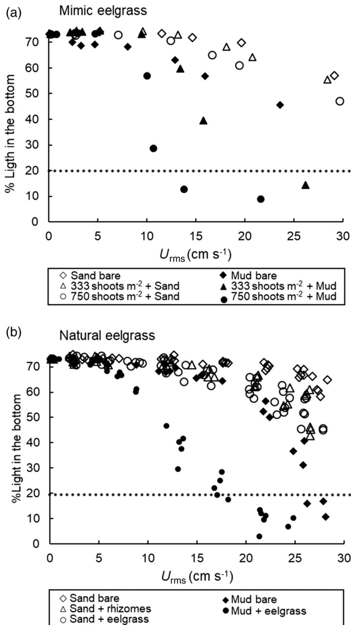
Fig. 4. Percentage of surface light reaching the bottom with increasing flow orbital velocities ( U_{rms} , cm s -1 ) for (a) mimic eelgrass and (b) natural eelgrass. The dot line indicates the minimum light requirement for eelgrass growth (20%).
