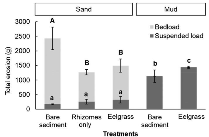
Fig. 5. Total erosion (g) in the form of bed load and suspended load for sandy and muddy trials after 56 min of wave exposure (mean ± SD). Significant differences in the bed load of sandy treatments are indicated by upper case letters and differences in the suspended load between all the treatments are indicated by lower case letters (Tukey’s HSD, p < 0.05 ). Bed-load erosion in muddy sediment is negligible. Total erosion as suspended load (g) was extrapolated from the turbidity (mg L -1 ) at the end of the trials to the volume of water contained in the flume, assuming that the turbidity was homogeneous in the whole flume.
